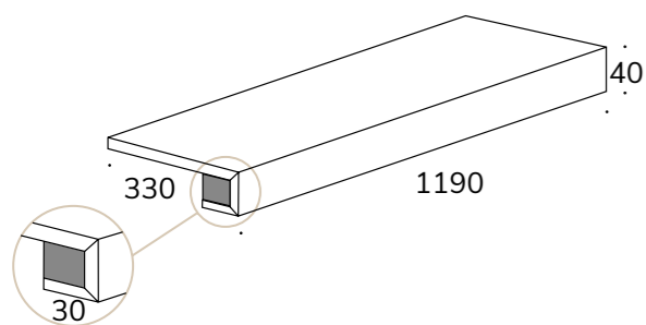
Costa retta 120
