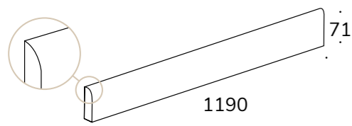
Skirting Battiscopa 120
